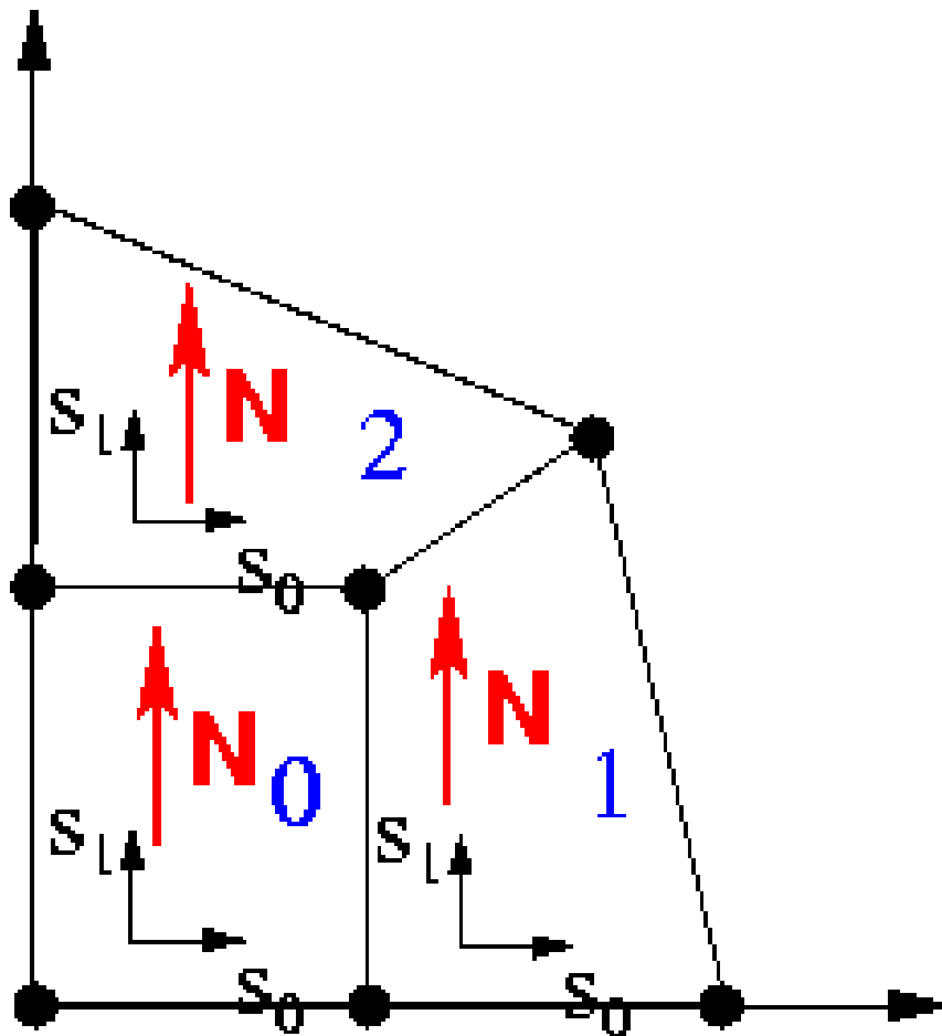
Figure 1.1 Mesh consisting of three RefineableQElements <2>/ QuadTrees . Element/ QuadTree numbers are blue, and the QuadTree 's `northern' direction is indicated by the red arrows. The QuadTrees are combined into a QuadTreeForest , which establishes their adjacency ( QuadTree 2 is QuadTree 0 's northern neighbour etc.) and their relative orientation ( QuadTree 1 's North coincides with QuadTree 2 's West, etc.) Note that the RefineableQElement <2>'s local coordinates s_0 and s_1 are aligned with the QuadTree 's W-->E and S-->N directions, respectively.
