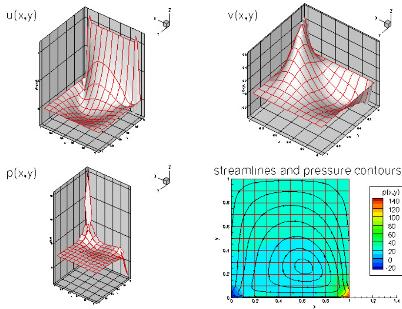
Figure 1.1 Plot of the velocity and pressure fields for Re=100 computed with Cruzeix-Raviart (Q2P-1) elements.
